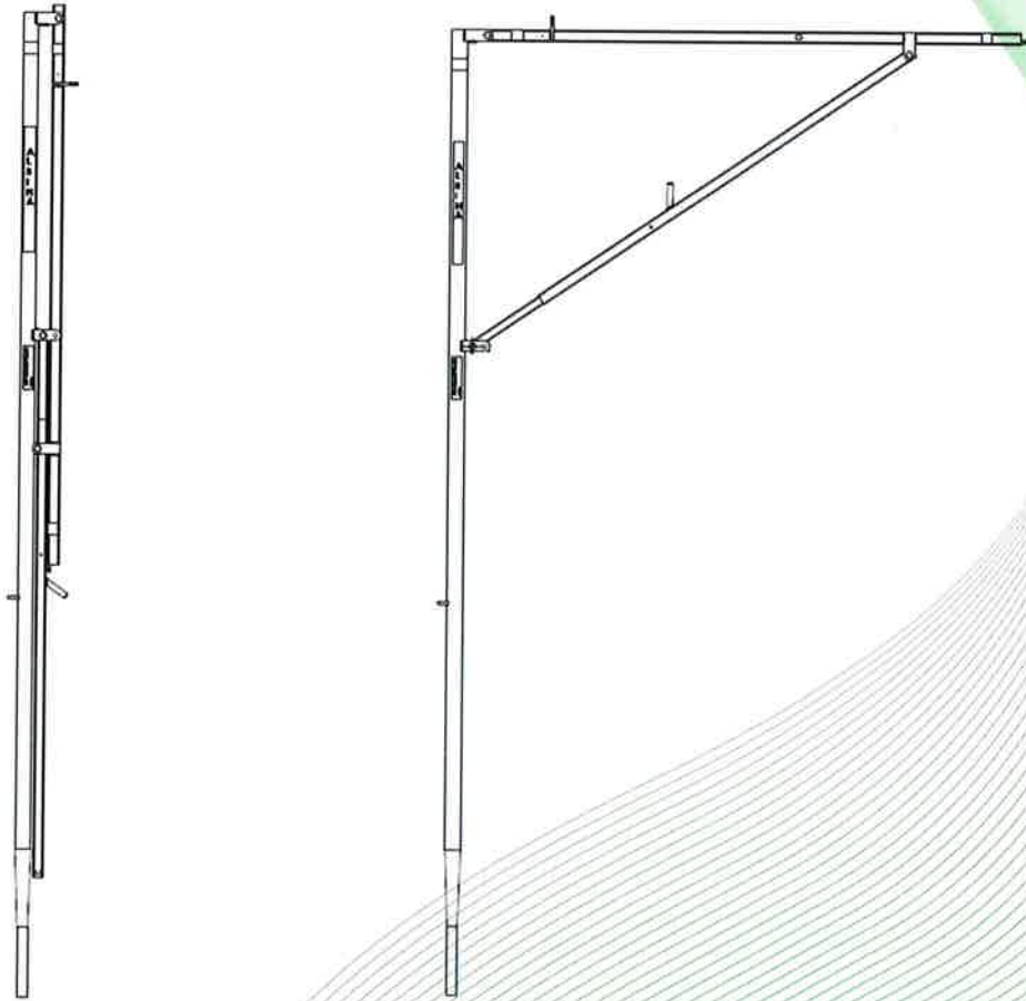
Fig. 1: Anchor device, type: Alsipercha
