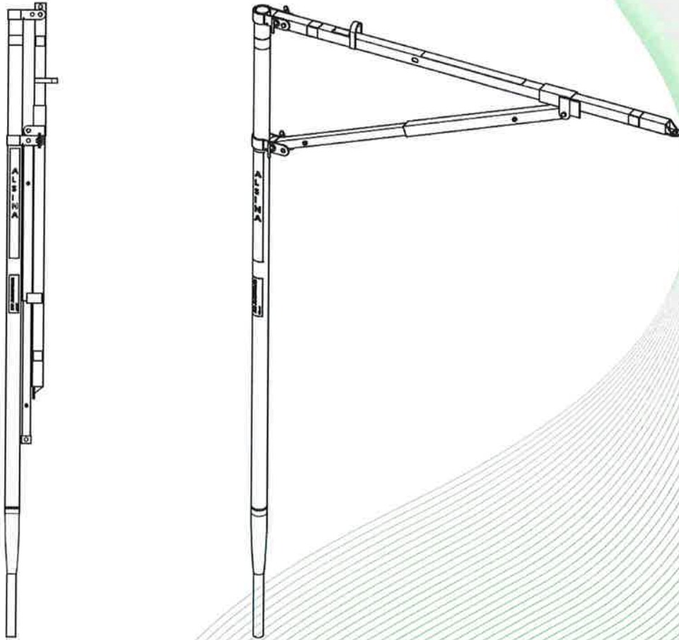
Fig. 1: Anchor device, type: AluPercha
